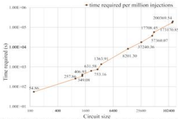
Fig. 2. The time required to SEE HDL simulations for ISCAS89 benchmark circuits.
